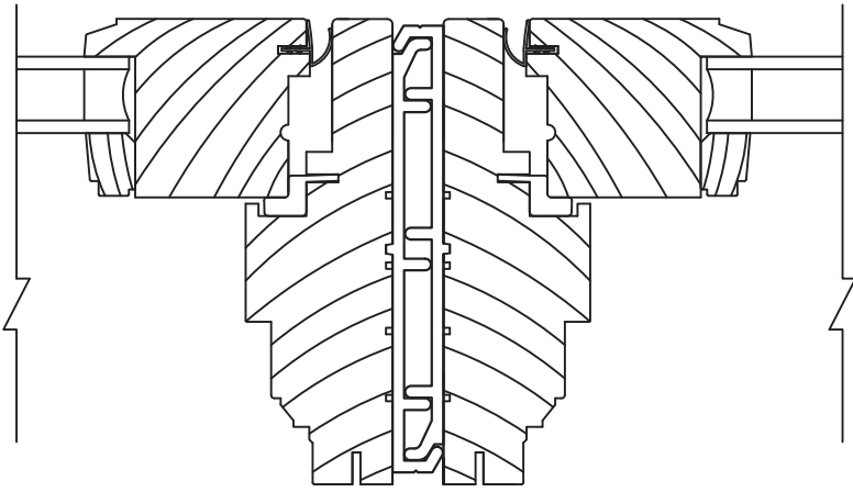
wood casement example
